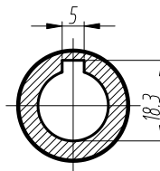
标准轴 Standard output shaft
